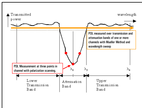
Figure 12: Measuring PDL over wavelength with polarization scanning and Mueller method.
