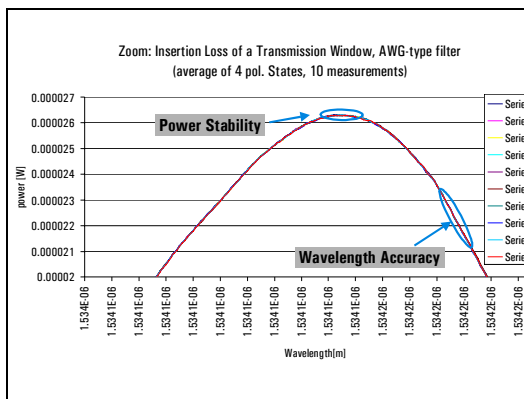
Figure 10: Evaluating the measurement setup includes wavelength repeatability and power stability.
