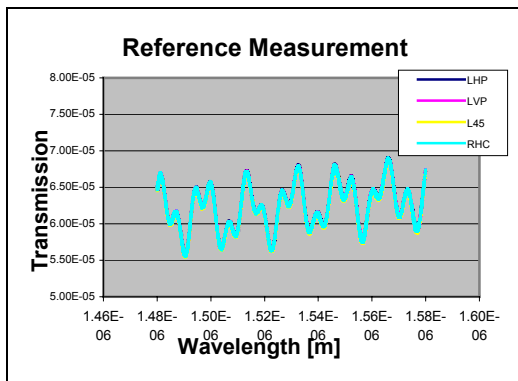
Figure 13: Müller method: Periodic variation in output power of the polarization controller.
