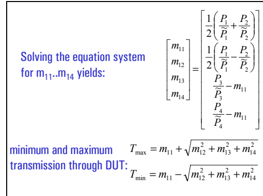
Figure 9: Calculation of minimum and maximum transmission.
