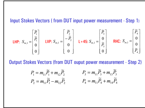
Figure 8: With the power measurement results, a system of linear equations can be solved.
