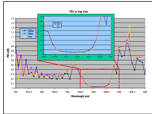
Figure 5: Polarization Scanning with three different averaging times: 100us, 1ms, and 10ms.
